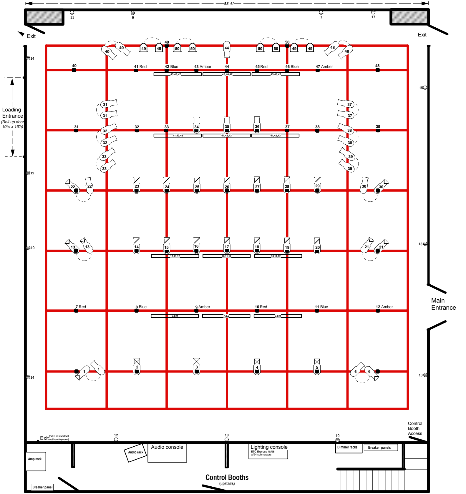
McCoy Studio Theater at the Maui Arts & Cultural Center Lighting Grid 1&1/2" Pipe grid is 20'6" from stage floor RC 8-07
